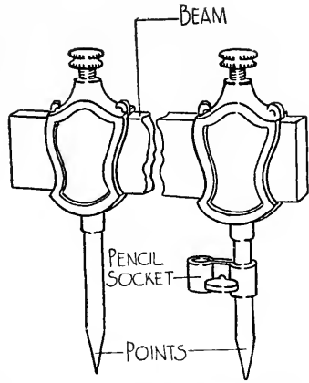
FIG. 44. TRAMMEL POINTS OR BEAM COMPASS.
